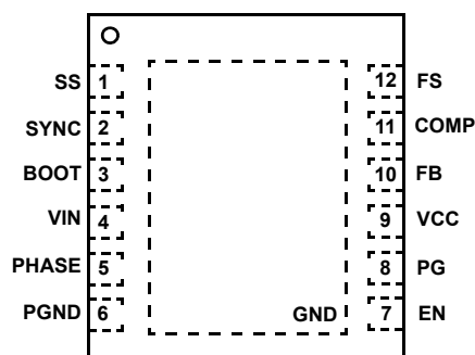
ISL85410 (12 LD 4X3 DFN) TOP VIEW
